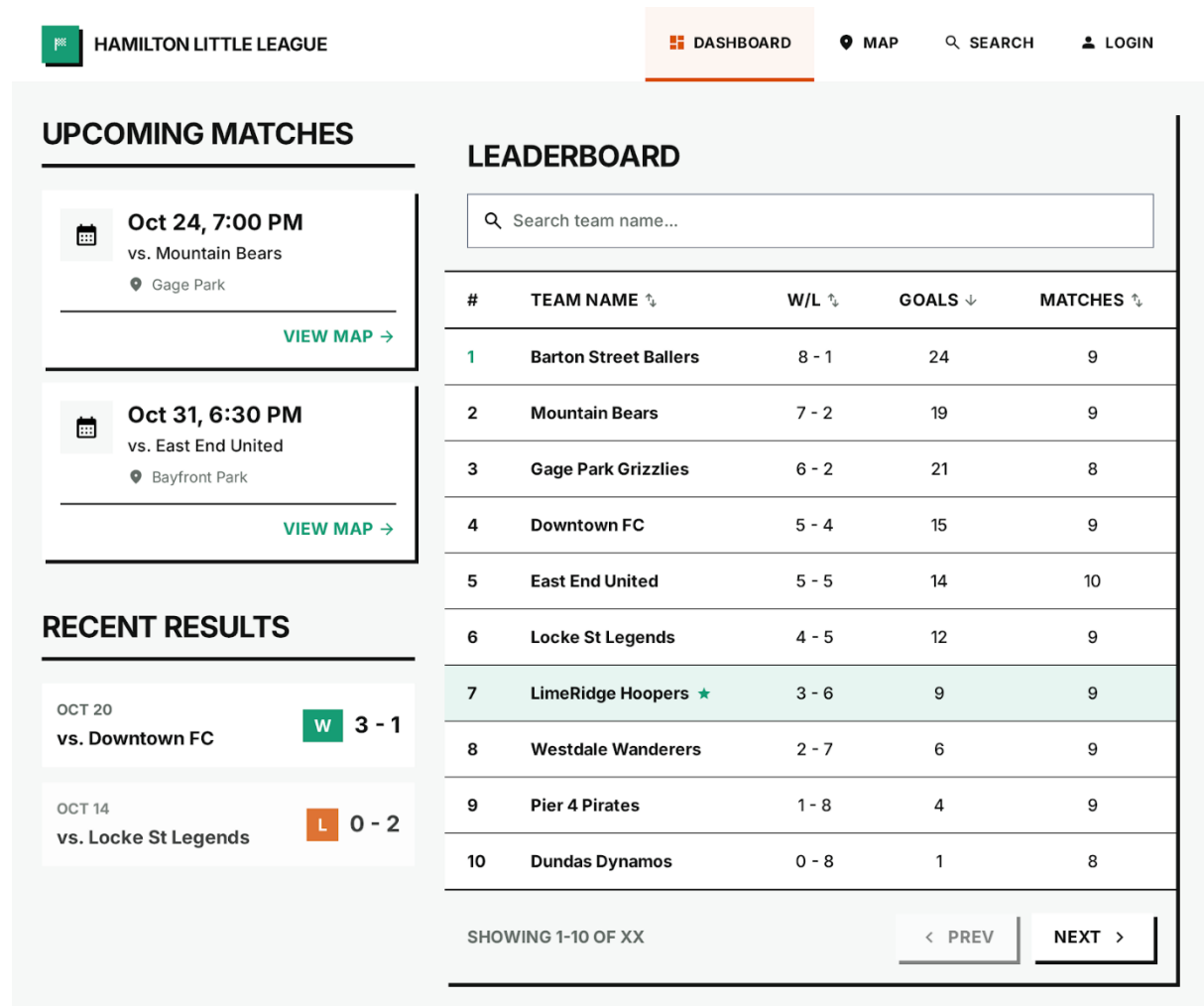
Figure 4: Dashboard view which includes an onclick sort feature on table headers
