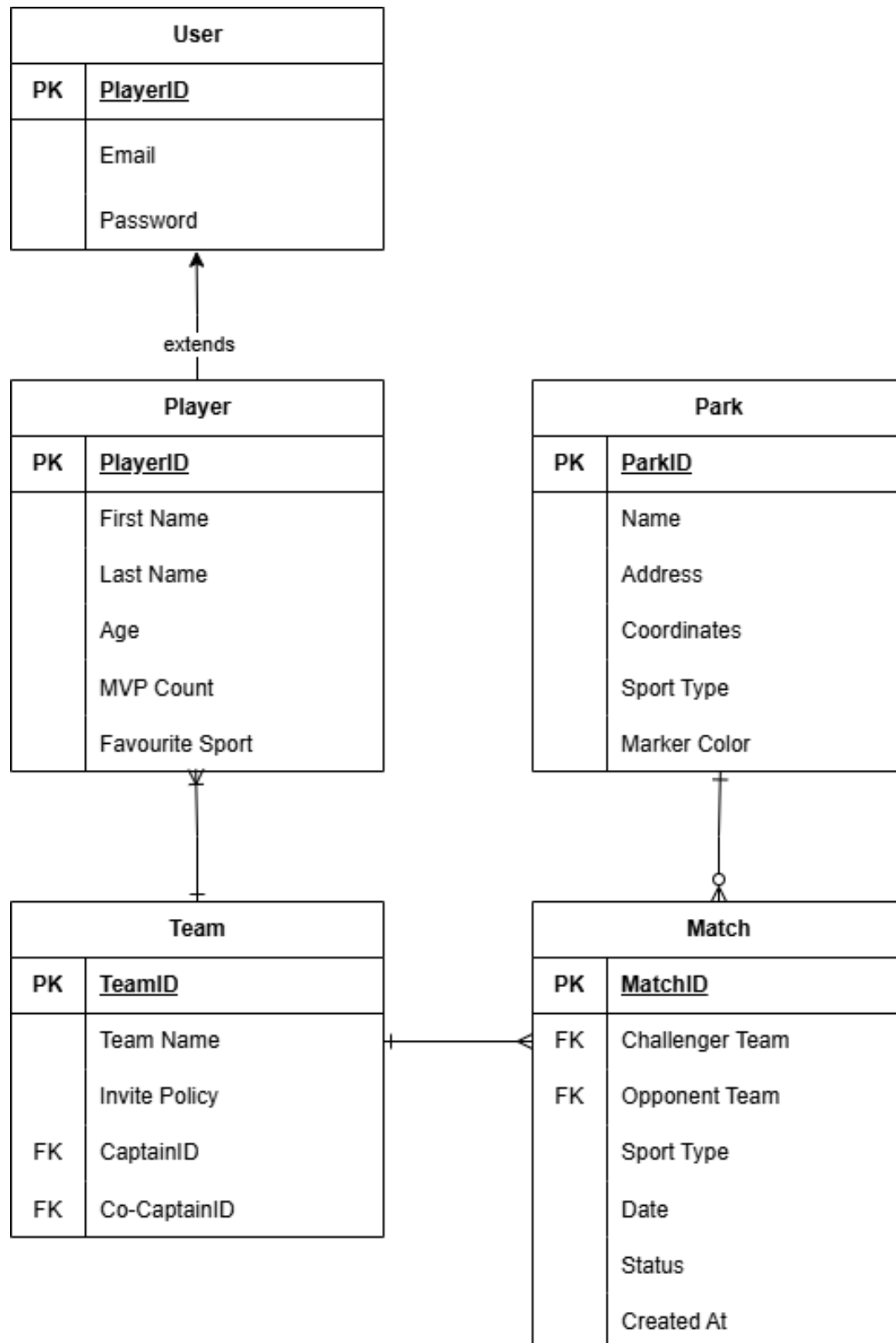
Figure 1: The ERD of the System
